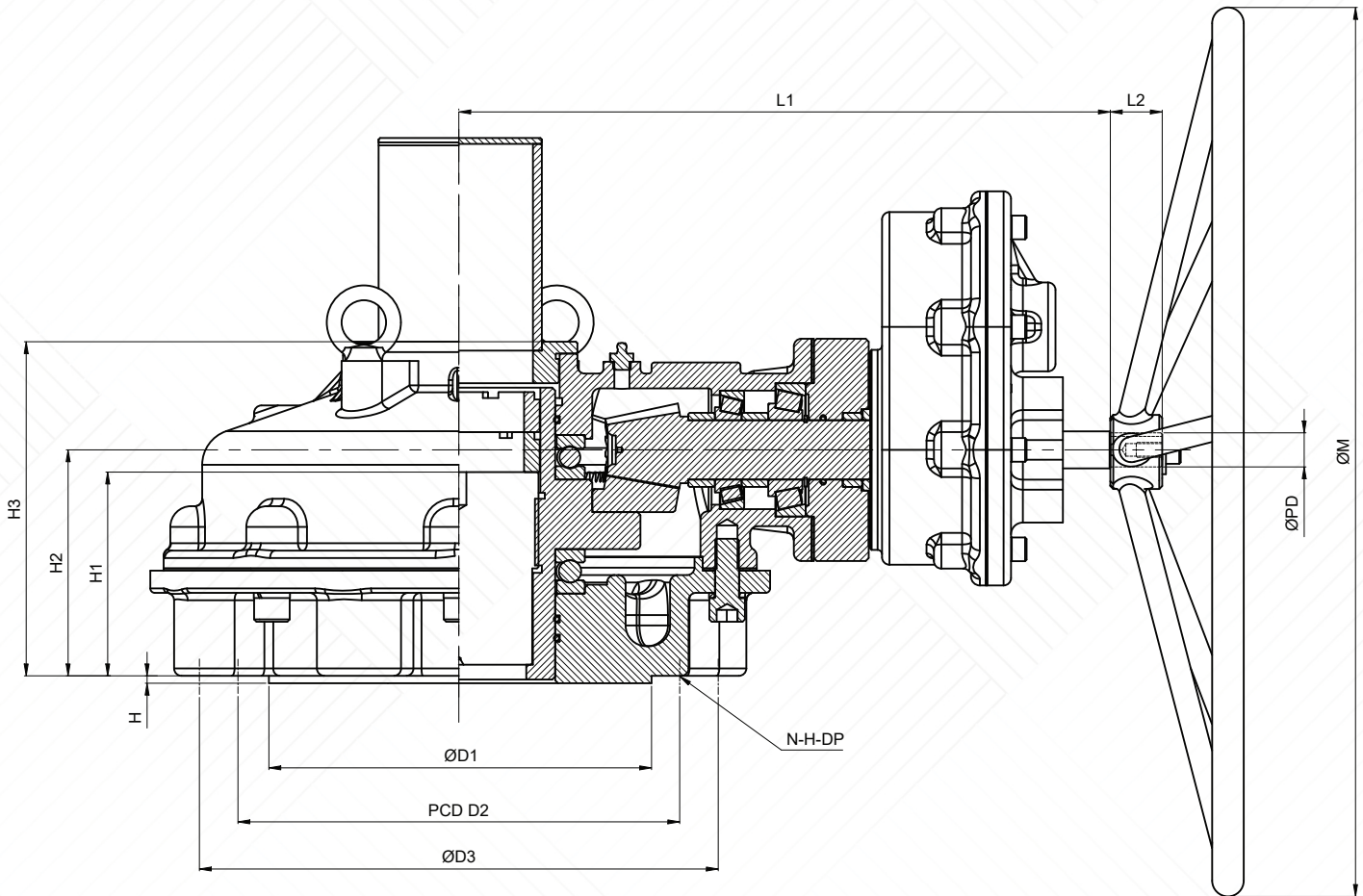
ISO 5210 Flange Mounting Details
