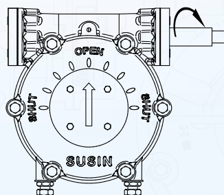
RH - Clockwise to Close
